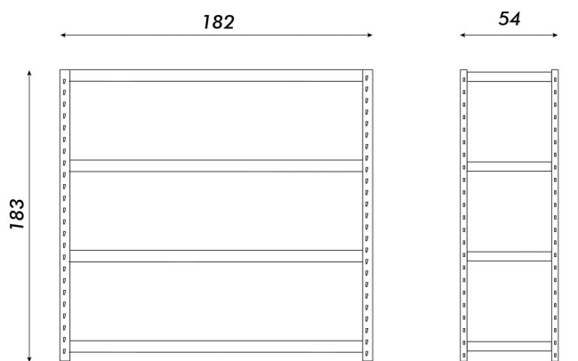
Vista frontal
